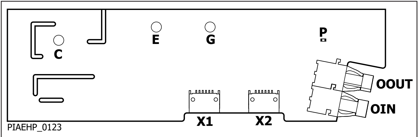
Figure 2. 1SP0630V2M1R Interfaces.
