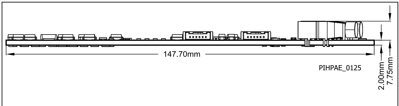
Figure 9. Side View.
