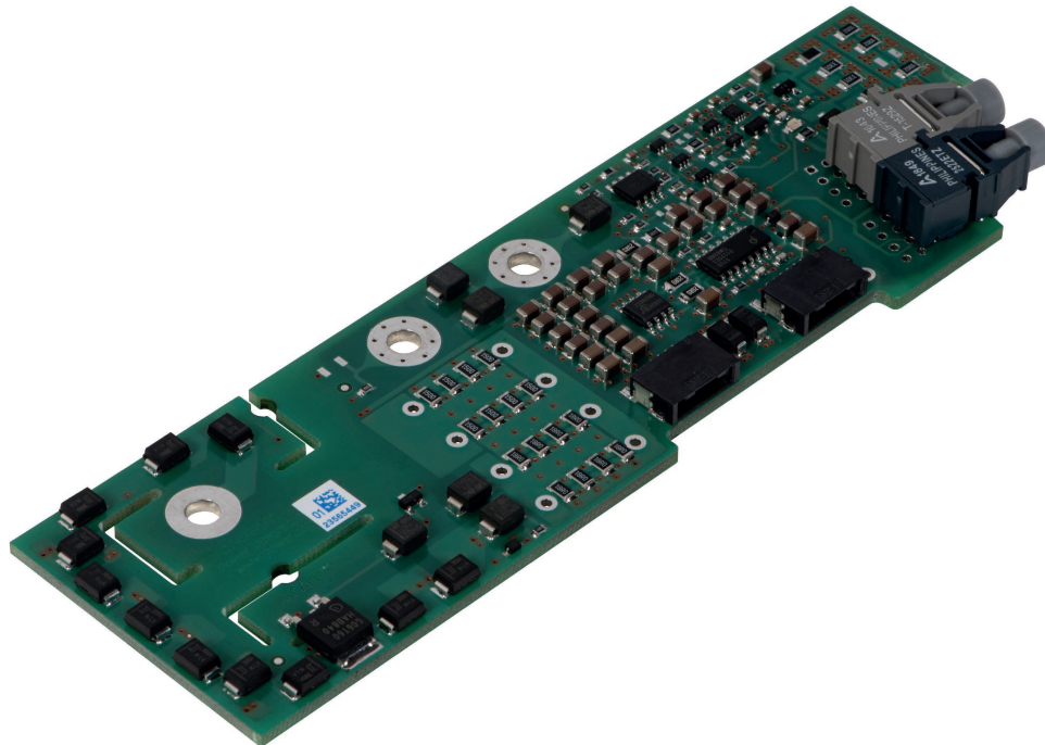
Figure 1. Board Photo of 1SP0630V2M1R.
